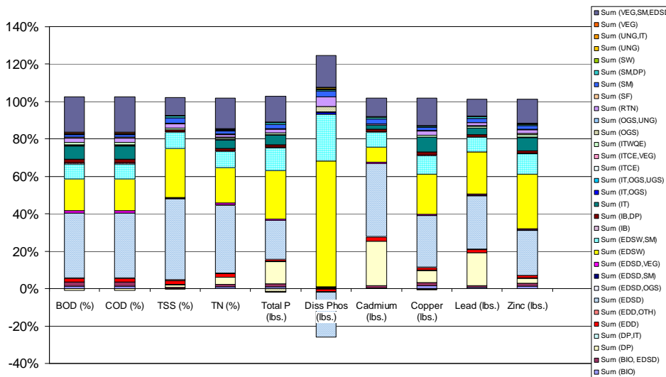
Figure 9-1. Percent pollutant removal by BMP type for Frederick County outfalls based on the Simple Method
